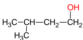
alcohol primario
